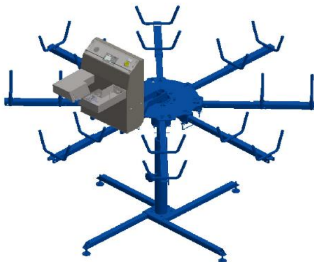
EXAMPLE OF A POSSIBLE COMBINATION BETWEEN A COUNTING DEVICE AND A ROTATING CAROUSEL
