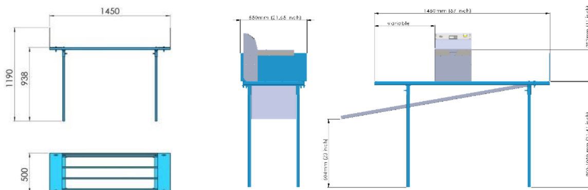
Dimensions-V01
